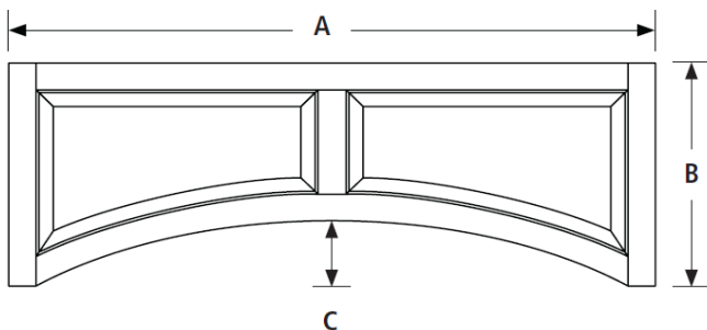
RAISED PANEL
