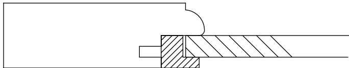
1/4" GLASS RETAINER (PRO287)
