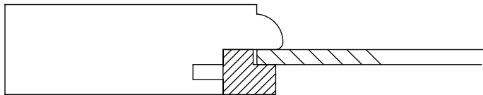
1/8" GLASS RETAINER (PRO288)
