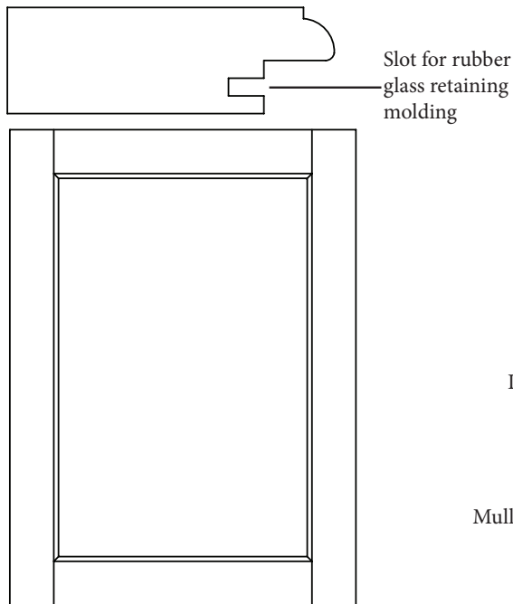
FRAME ONLY
