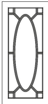
ELLIPTICAL OFFSET 54" MAX HEIGHT
